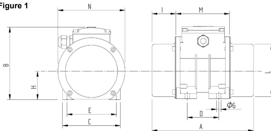
DIMENSIONS (mm)
